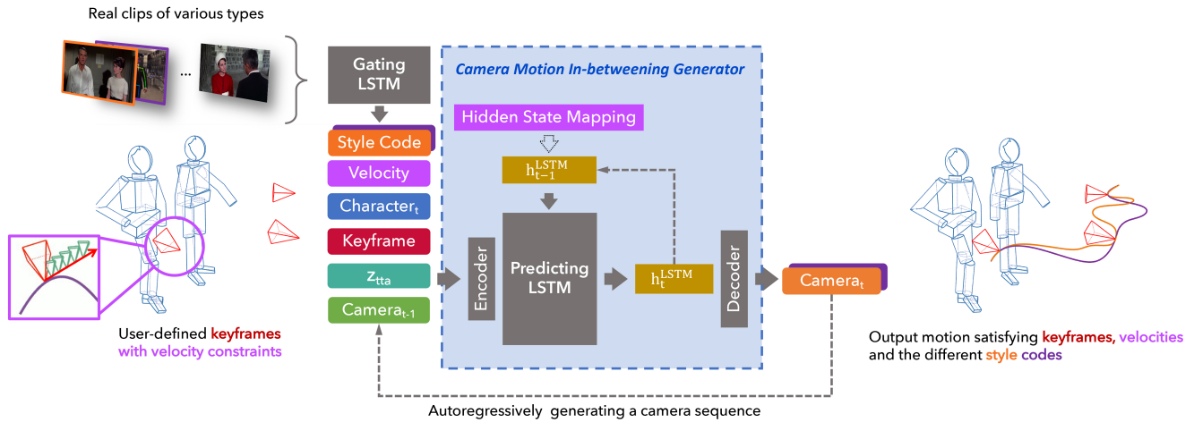
Fig. 2. Our proposed framework for learning camera together with keyframe constraints composed of a camera behavior extractor (Gating LSTM), which extracts camera behaviors from reference clips (from Charade , 1963), and a camera motion generator, which generates camera trajectories that both meet the camera behaviors and required keyframe constraints, speed and directions.
